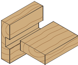
Right-angle joint
